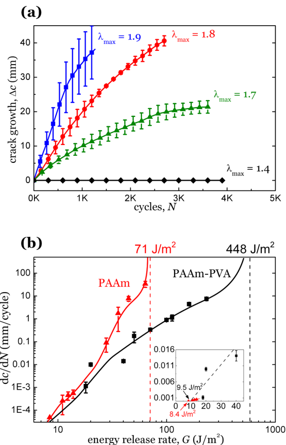
Figure 4. Fatigue fracture of the PAAm-PVA hydrogel. (a) The crack growth with cycles in a PAAm-PVA hydrogel under different applied stretch \lambda_{\max} . (b) The crack growth per cycle dc/dN as a function of the energy release rate G for the PAAm hydrogel (data extracted from ref 58) and the PAAm-PVA hydrogel. Inset: linear regression of the first three points of experimental data. Vertical dashed lines: the experimentally measured bulk fracture toughness under the loading rate 0.4 s -1 . Solid curves: guiding lines of the data points. All the data represent the mean and standard deviation of three experimental results.
