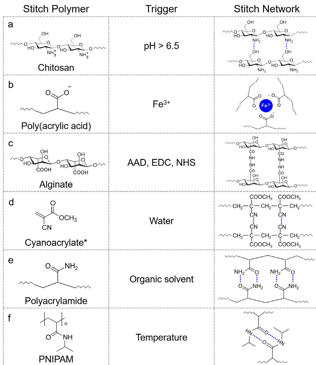
Fig. 5. Examples of topohesives for wet, elastic, strong adhesion. A trigger gelsates the stitch polymer into the stitch network. Chitosan crosslinks into a noncovalent network by hydrogen bonds at pH > 6.5. Acrylic acid crosslinks into a noncovalent network by ionic bonding with iron (III) ions. Alginate crosslinks into a covalent network by chemical crosslinkers. Cyanoacrylate polymerizes in the presence of water and subsequently crosslinks into a noncovalent glassy network. It is possible that topohesives can be made using PAAm and PNIPAM stitch polymers triggered by exposure to an organic solvent and high temperature, respectively. *Cyanoacrylate monomers form stitch polymers.
